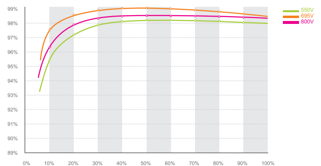
Growatt 50000TL3-S efficiency
